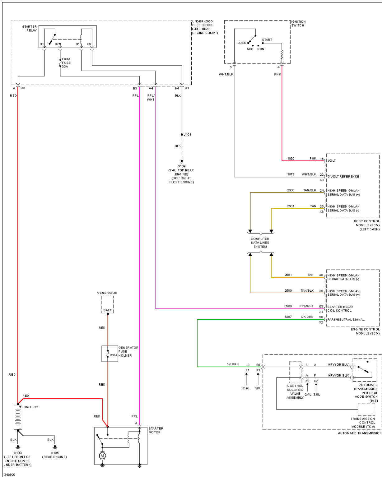
Fig. 72: Starting Circuit
