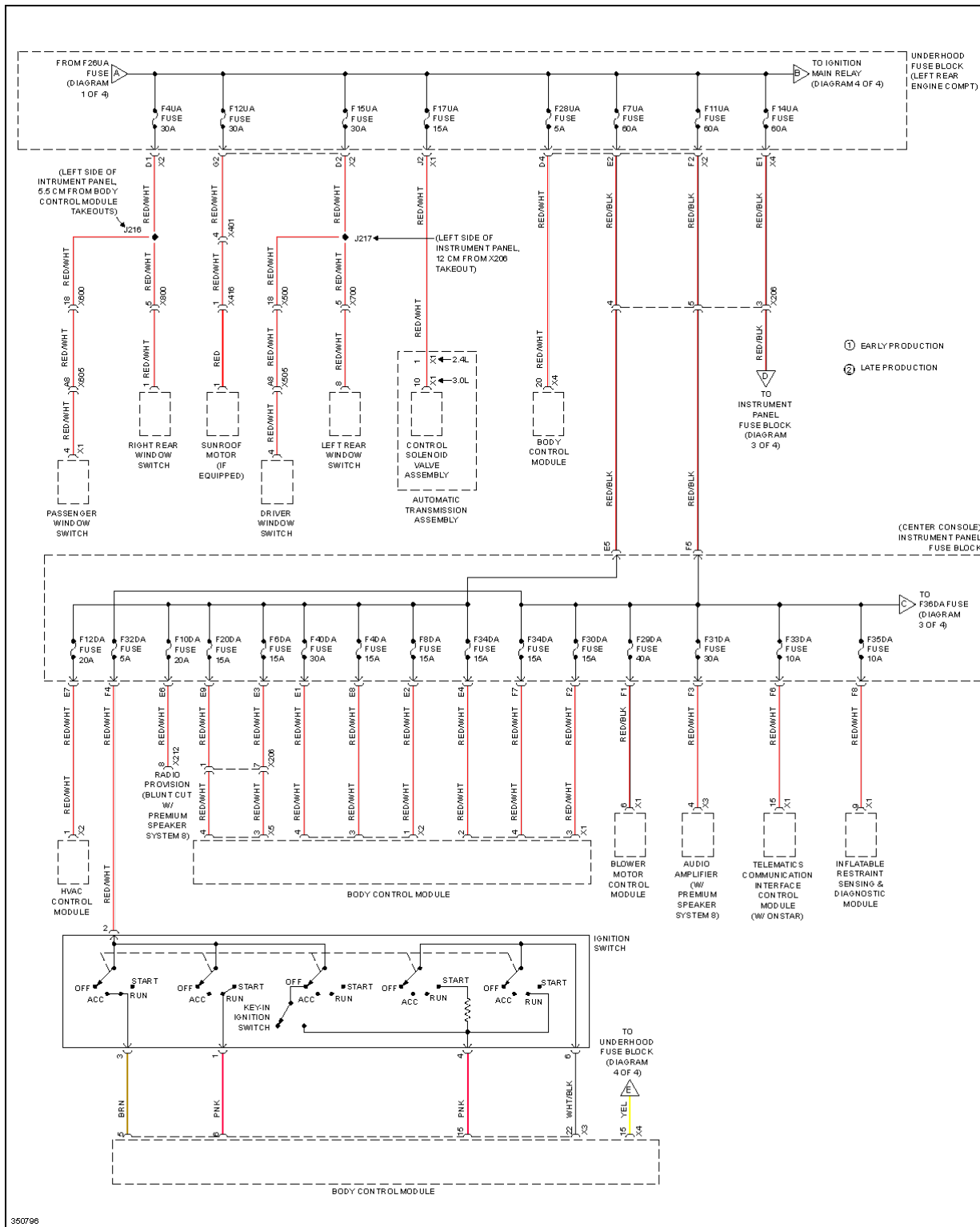
Fig. 50: Power Distribution Circuit (2 of 4)
