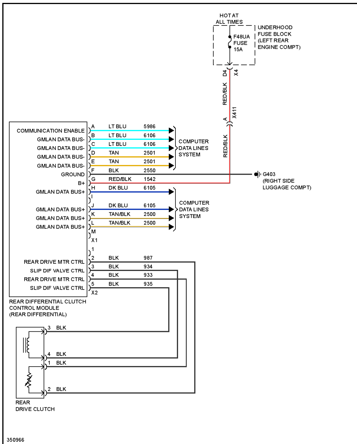
Fig. 76: 2.4L VIN C, Rear Differential Lock Circuit
