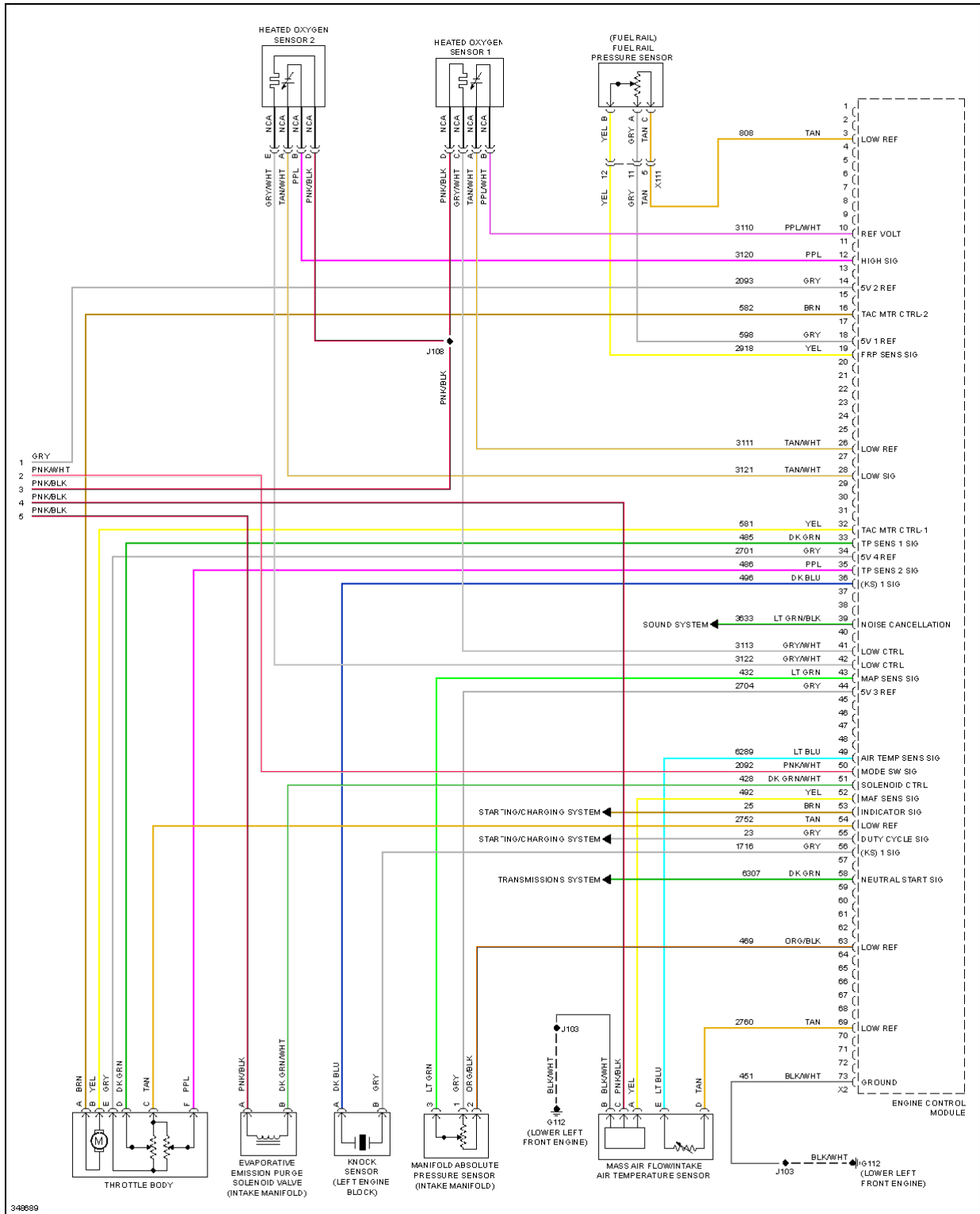
Fig. 23: 2.4L VIN C, Engine Performance Circuit (5 of 5)
