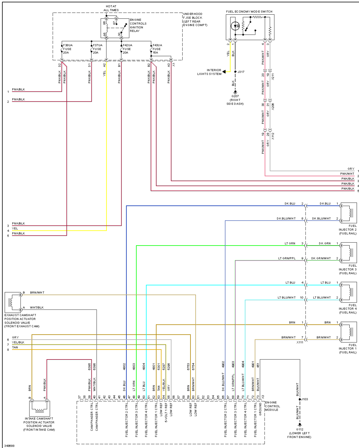
Fig. 22: 2.4L VIN C, Engine Performance Circuit (4 of 5)
