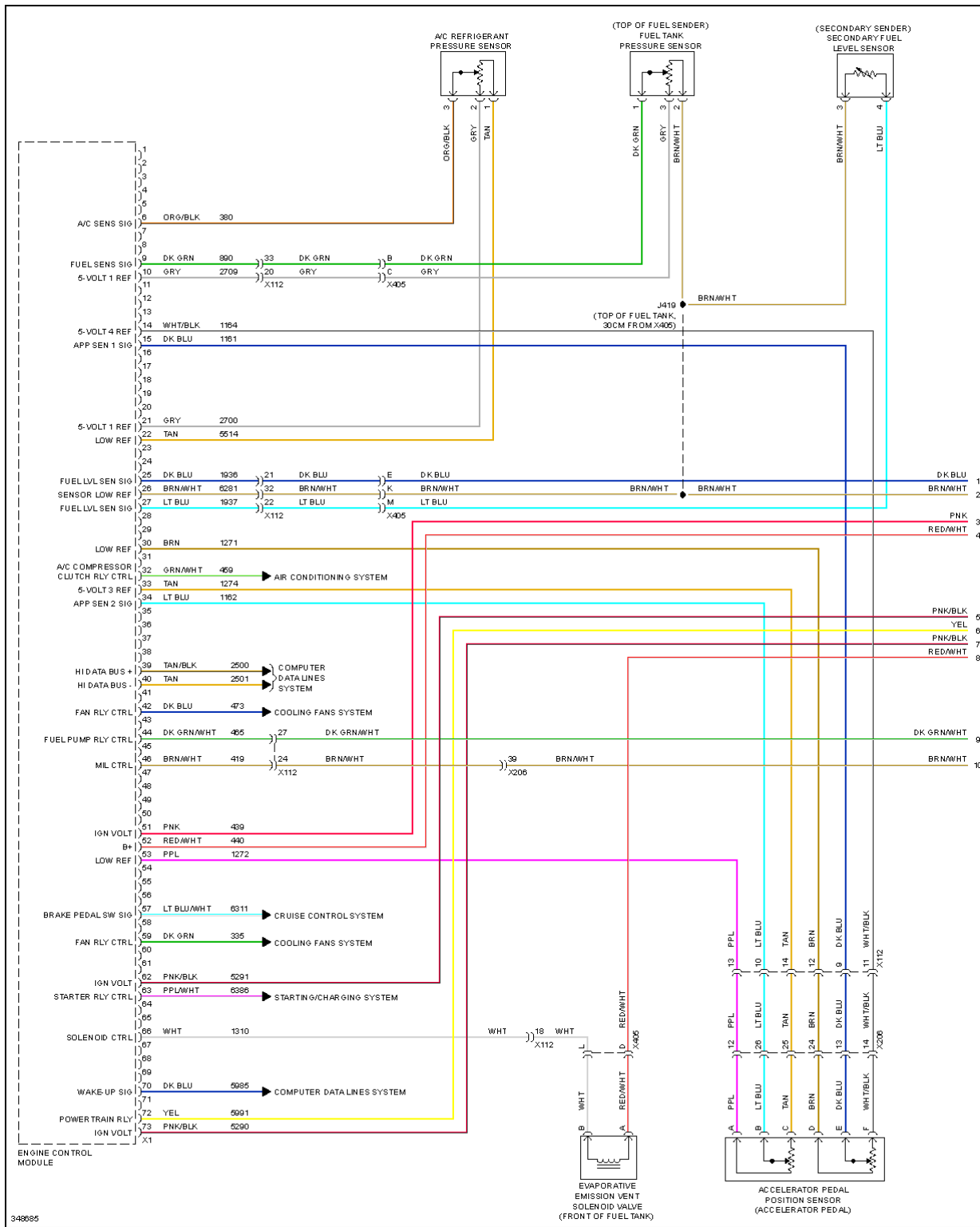
Fig. 19: 2.4L VIN C, Engine Performance Circuit (1 of 5)
